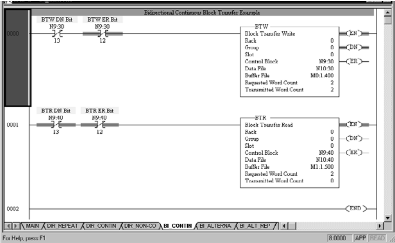
Figure 8.5 Bi-directional Continuous
