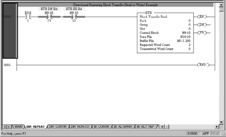
Figure 8.4 Directional Continuous
