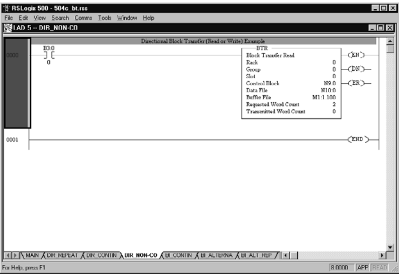
Figure 8.2 Directional
